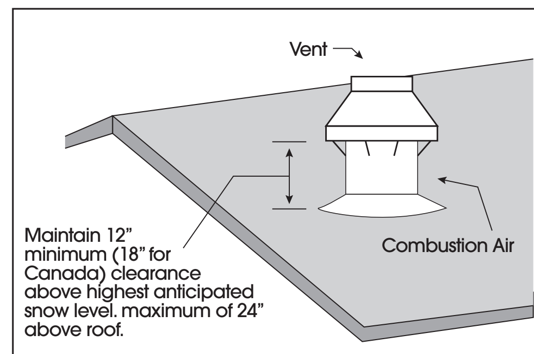
Figure 2-Typical Roof Installation
