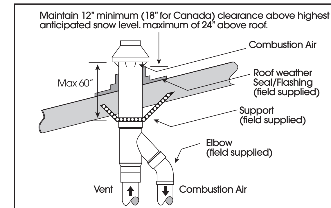
Figure 3-Typical Roof Install
