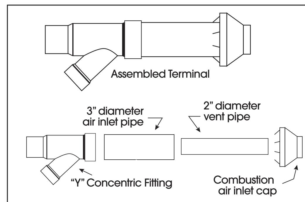
Figure 1-Vent Terminal Assembly
